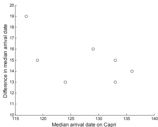
Figure 5. The differences in median arrival dates between Ottenby and Capri plotted against the species-specific arrival dates on Capri. r = -0.57 , P = 0.18
